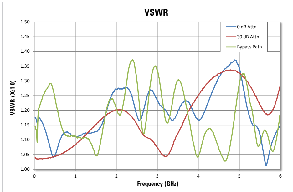
Figure 10. Measured VSWR from 1 MHz to 6 GHz.
